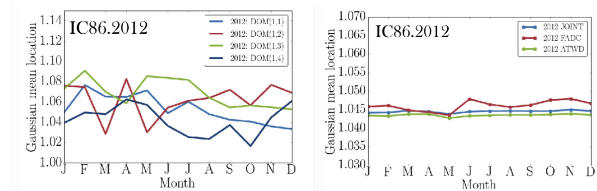
Figure 1: The change in the fitted location of the Gaussian mean throughout the course of an entire season. The paper describes the fitting procedure for the ATWD, feel free to ignore the FADC line. It's also worth noting that since these are seasonal fits, the statistics used is 1/12th that of every year. Left is the result of four DOMs throughout IC86.2012, Right is the average over the full detector.
